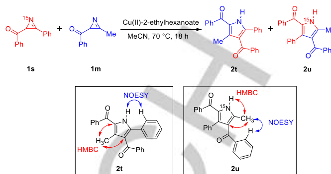
Scheme 7. Isolated cross coupling products and determination of their structure via NMR experiments.
