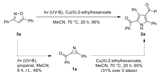
Scheme 3. Comparison of the one-pot synthesis of tetrasubstituted pyrroles from isoxazoles with a divided reaction setup.
