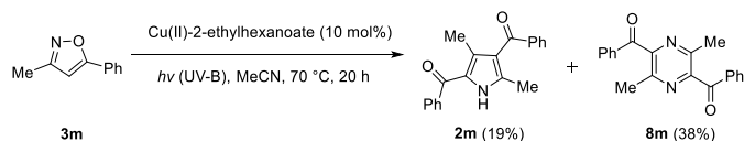
Scheme 6. Isolated products of the dimerization reaction applying standard conditions on isoxazole 3i .
