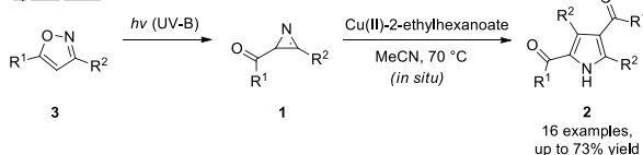
Scheme 1. a) iron dichloride catalyzed dimerization of isoxazoles forming 2,4-alkoxycarbonylpyrroles b) photochemically in situ -generated 2-acylazirines in the synthesis of imidazoles and 2,4-dialkylpyrroles c) copper(II)-2-ethylhexanoate catalyzed dimerization of in situ generated 2-acylazirines. [7–9]
