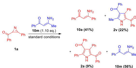
Scheme 11. Product distribution using the standard conditions with an external enaminone; Yields were calculated using phenanthrene as an internal standard ( ^1\text{H-NMR} ).
