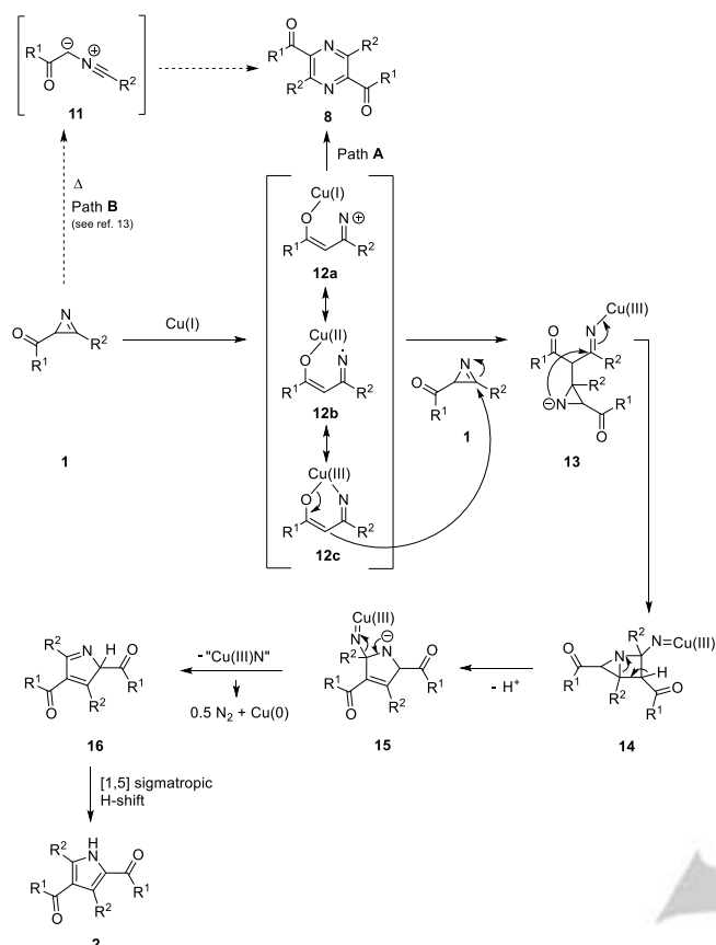
Scheme 8. Plausible mechanism for the formation of the tetrasubstituted pyrroles 2 . (For the simplicity, the ligands/counterions of the copper catalyst are not shown).
