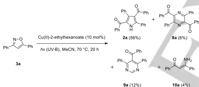
Scheme 4. Isolated compounds of the upscaled one-pot reaction.
