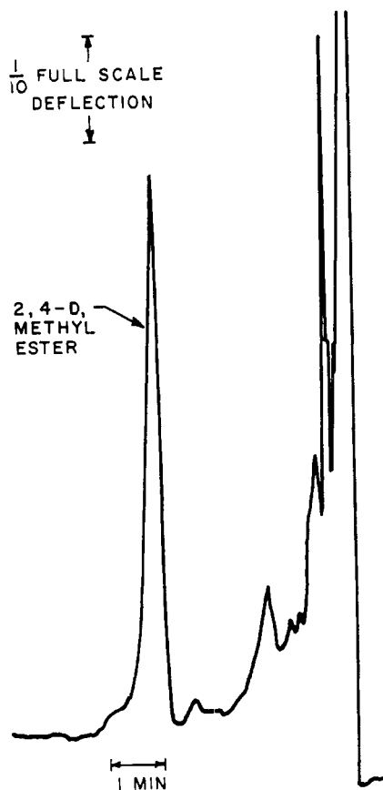
Figure 1. Chromatogram of 2,4-D methyl ester in oranges extract
