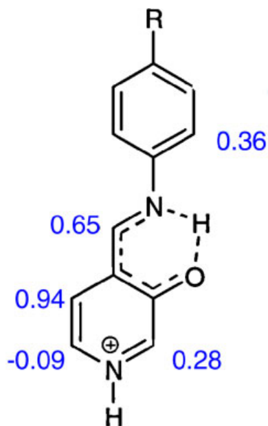
Figure 1. Protonation effects in the ^1\text{H} -NMR chemical shifts [ \Delta\delta(\text{TFA}-\text{CDCl}_3) ] of compounds 8–12 . This figure is available in colour online at www.interscience.wiley.com/journal/poc
