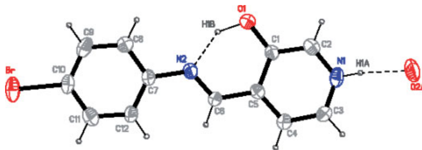
Figure 7. ORTEP plot of ( E )-4-[(4-bromophenylimino)methyl]-3-hydroxypyridinium tetrafluoroborate ( 11H + BF 4 - ) with thermal ellipsoids at 30% probability. The BF 4 anion is omitted for clarity purposes
