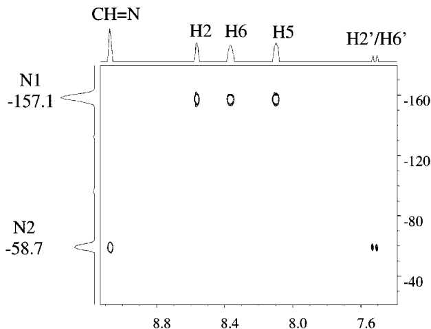
Figure 6. gs-HMBC ^{15}\text{N} -NMR of ( E )-4-[(4-methoxyphenylimino)methyl]-3-hydroxypyridinium tetrafluoroborate ( 10H + BF 4 - ) in DMSO- d 6
