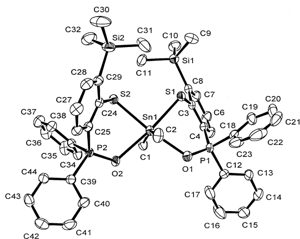
Fig. 2. Molecular structure of [\text{Me}_2\text{Sn}\{2-(\text{Ph}_2\text{PO})-6-(\text{Me}_3\text{Si})\text{C}_6\text{H}_3\text{S}\}_2] (3).
