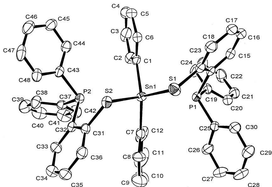
Fig. 1. Molecular structure of [\text{Ph}_2\text{Sn}\{2-(\text{Ph}_2\text{P})\text{C}_6\text{H}_4\text{S}\}_2] (2).
