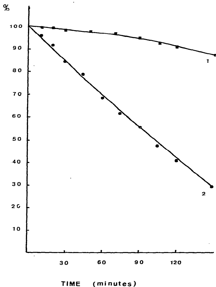
Fig. 4. Hydrogenation of trans -1,3-pentadiene catalysed by a toluene solution of \text{Rh}_2\text{Cl}_2(\text{CO})_4 in the presence of \text{PPh}_3 under 1 atm \text{H}_2 at 70^\circ\text{C} . Molar ratio [\text{Rh}_2\text{Cl}_2(\text{CO})_4]/[\text{PPh}_3] = 1 . Ordinate: percentage of residual pentadiene; abscissa: time in minutes. Curve 1: no thermal treatment of the solution containing \text{Rh}_2\text{Cl}_2(\text{CO})_4 and \text{PPh}_3 before the addition of substrate. Curve 2: solution containing \text{Rh}_2\text{Cl}_2(\text{CO})_4 and \text{PPh}_3 heated at 70^\circ\text{C} for 2 hours before the addition of substrate.
