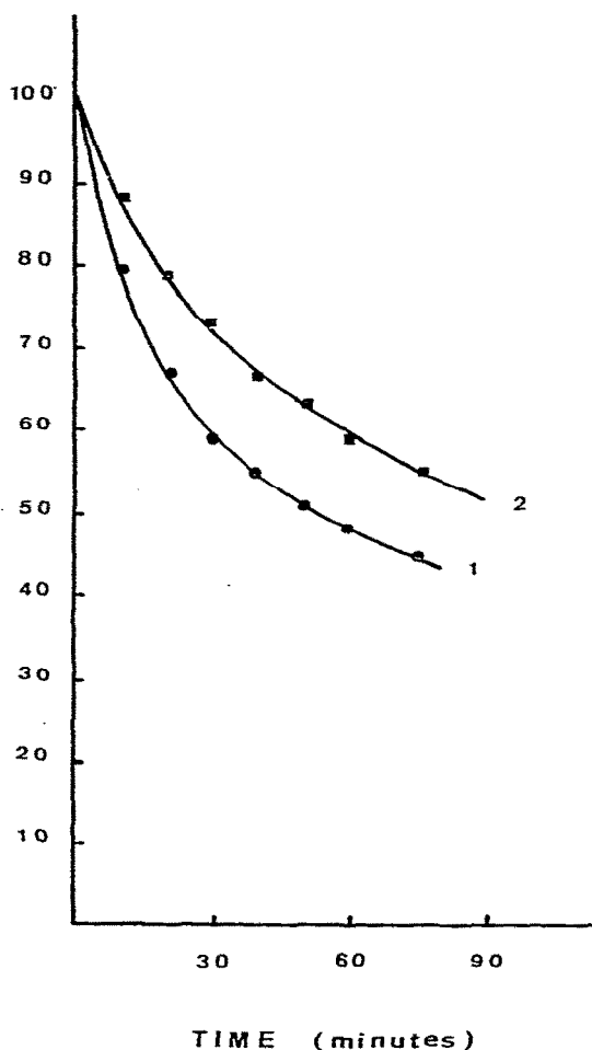
Fig. 3. Hydrogenation of trans -1,3-pentadiene catalysed by \text{Rh}_2\text{Cl}_2(\text{CO})_4 supported on \text{Al}_2\text{O}_3 under 1 atm \text{H}_2 at 70^\circ\text{C} . Ordinate: percentage of residual trans -1,3-pentadiene; abscissa: time in minutes. Curve 1: first cycle; curve 2: second cycle. For further explanation, see text.
