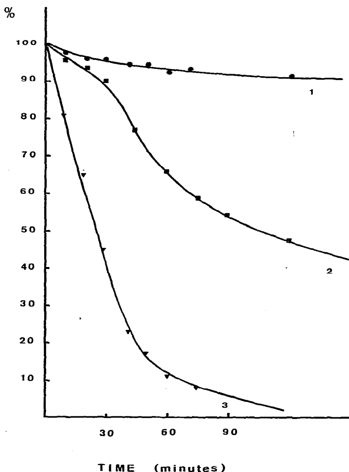
Fig. 5. Hydrogenation of trans -1,3-pentadiene catalysed by \text{Rh}_2\text{Cl}_2(\text{CO})_4 anchored on \text{Al}_2\text{O}_3 , in the presence of \text{PPh}_3 under 1 atm \text{H}_2 at 70°C. Molar ratio [\text{Rh}_2\text{Cl}_2(\text{CO})_4]/[\text{PPh}_3] = 1 . Ordinate: percentage of residual pentadiene; abscissa: time in minutes. Curve 1: addition of \text{PPh}_3 followed the anchorage of \text{Rh}_2\text{Cl}_2(\text{CO})_4 on \text{Al}_2\text{O}_3 ; curve 2: \text{PPh}_3 and \text{Rh}_2\text{Cl}_2(\text{CO})_4 mixed immediately before the anchorage; curve 3: \text{Al}_2\text{O}_3 kept in contact with \text{PPh}_3 for 10 hours before the anchorage of \text{Rh}_2\text{Cl}_2(\text{CO})_4 .
