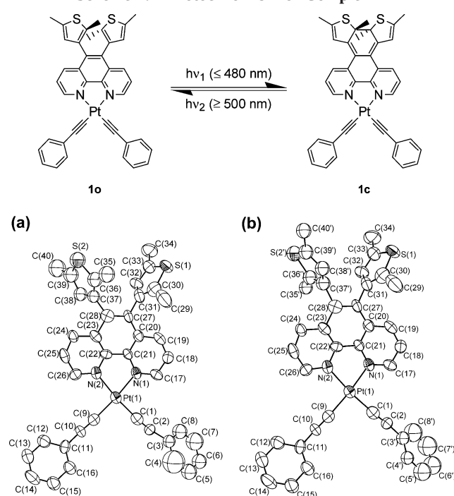
Figure 1. Perspective drawings of 1 as the parallel (a) and antiparallel (b) conformers with atomic numbering scheme. Hydrogen atoms have been omitted for clarity. Thermal ellipsoids are shown at the 30% probability level.
