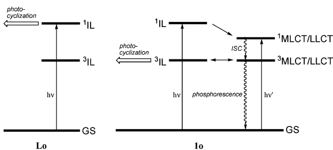
Scheme 2. Qualitative Energy State Diagram of L and 1
