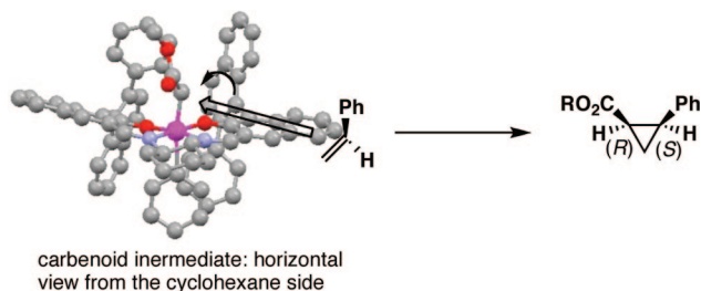
Figure 4. Explanation of the stereochemistry of the aryliidium–salen-catalyzed asymmetric cyclopropanation, based on the optimized structure of the phenyliridium–salen carbenoid intermediate.
