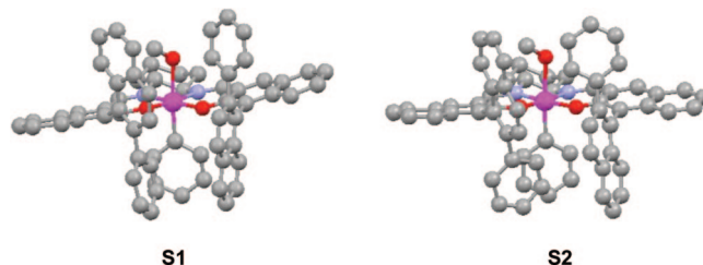
Figure 3. X-ray structures of the two stereoisomers of complex 4 . Horizontal view from the binaphthyl side. Ir, violet; C, black; N, blue; O, red.
