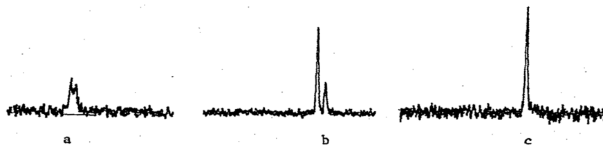
Fig. 2. ^{19}\text{F} spectrum of [(\text{C}_6\text{H}_5)(p\text{-FC}_6\text{H}_4)\text{SbCl}_2]_2\text{O} , (a) uncrySTALLIZED product; (b) the more soluble fraction after partial fractional crystallization; (c) the pure more-soluble product showing a single ^{19}\text{F} peak.
