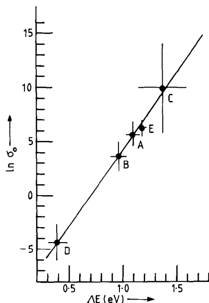
Fig. 7. Plot of \ln \sigma_0 against \Delta E (with \sigma_0 and \Delta E defined by the equation \sigma = \sigma_0 \exp(-\Delta E/2kT) for the temperature dependence of conductivity \sigma ) for the complexes, based on values of \sigma_0 and \Delta E for heating: A, \text{Mn}(\text{C}_{15}\text{H}_{23}\text{N})\text{Cl}_2 ; B, \text{Co}(\text{C}_{15}\text{H}_{23}\text{N})\text{Cl}_2 ; C, \text{Ni}(\text{C}_{15}\text{H}_{23}\text{N})\text{Cl}_2 ; D, \text{Cu}(\text{C}_{15}\text{H}_{23}\text{N})_2\text{Cl}_2 ; E, \text{Zn}(\text{C}_{15}\text{H}_{23}\text{N})_2\text{Cl}_2 . The line is fitted by least squares and has the equation \ln \sigma_0 = (14.3 \pm 0.6) \Delta E - (10.1 \pm 0.6) with \sigma_0 and \Delta E respectively in units of \Omega^{-1} \text{ m}^{-1} and eV.
