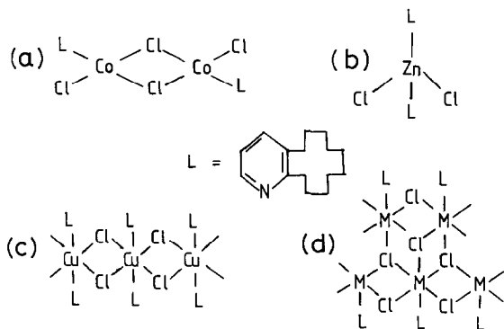
Fig. 1. Proposed stereochemistry of the metal complexes with cyclododecenopyridine (L): (a) \text{CoLCl}_2 ; (b) \text{ZnL}_2\text{Cl}_2 ; (c) \text{CuL}_2\text{Cl}_2 ; (d) \text{MLCl}_2 where \text{M} = \text{Mn} or \text{Ni} .
