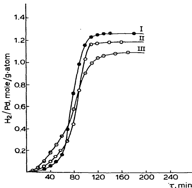
Fig. 1. Kinetic curves for the absorption of H_2 in toluidines. I. [(PPh_3)PdCl_2]_2 = 2.4 \times 10^{-3} mol/l, 50^\circ C , solvent m -toluidine. II. [(PPh_3)PdCl_2]_2 = 2.4 \times 10^{-3} mol/l, 50^\circ C , solvent o -toluidine. III. [(PPh_3)PdCl_2]_2 = 2.4 \times 10^{-3} mol/l, 50^\circ C , solvent p -toluidine.
