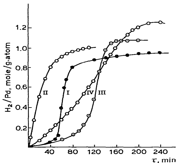
Fig. 2. Kinetic curves for the absorption of H_2 in aniline. I. [(PPh_3)PdCl_2]_2 = 2.4 \times 10^{-3} mol/l, 50^\circ C . II. [(PPh_3)PdBr_2]_2 = 2.4 \times 10^{-3} mol/l, 50^\circ C . III. [(PPh_3)PdCl_2]_2 = 2.4 \times 10^{-3} mol/l, 50^\circ C , volume ratio H_2 : Ar = 1 : 1 . IV. [(PPh_3)PdCl_2]_2 = 1.2 \times 10^{-3} mol/l, 50^\circ C . V. [(PPh_3)PdCl_2]_2 = 2.4 \times 10^{-3} mol/l, 50^\circ C , with addition of the hydrogenated complex. VI. [(PPh_3)PdCl_2]_2 = 2.4 \times 10^{-3} mol/l, 30^\circ C .
