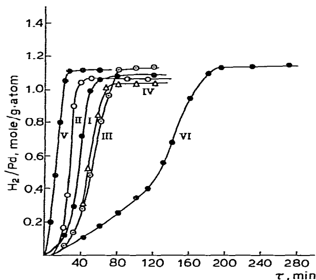
Fig. 3. Kinetic curves for the absorption of H_2 in aniline and biphenyl. I. [(PPh_3)_2Pd(Br)Ph] = 4.7 \times 10^{-3} mol/l, 50^\circ C , solvent biphenyl. II. [p(OPh)_3]_2PdCl_2 = 4.7 \times 10^{-3} mol/l, 50^\circ C , solvent aniline. III. [(PPh_3)_2Pd(Br)Ph] = 4.7 \times 10^{-3} mol/l, 70^\circ C , solvent aniline. IV. [(PPh_3)_2PdCl_2] = 4.7 \times 10^{-3} mol/l, 90^\circ C , solvent aniline.
