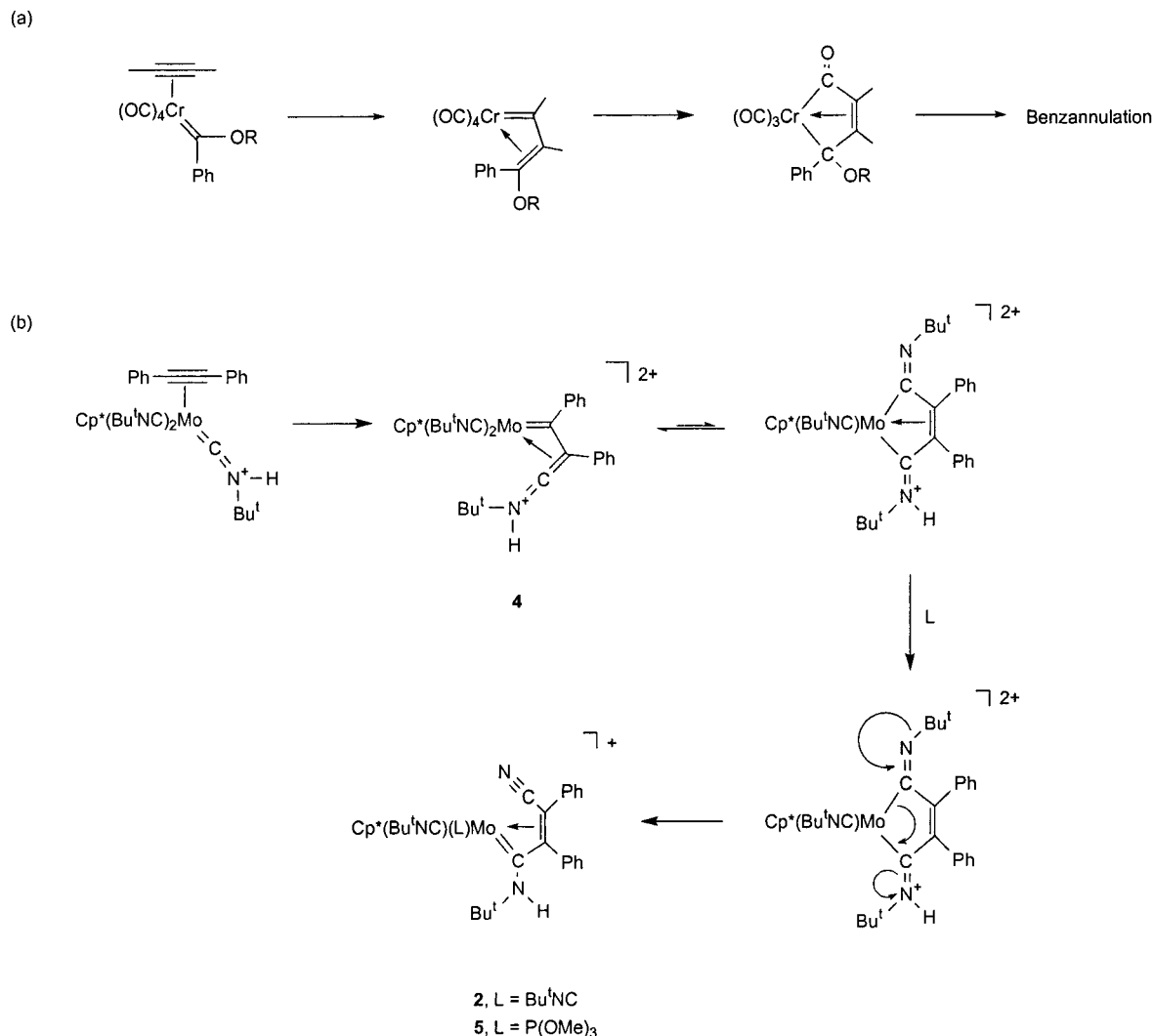
Scheme 4. (a) Initial Stages of the Dötz Reaction and (b) the Formation of 4 and Its Equilibrium with an Isomeric Metallacycle a
