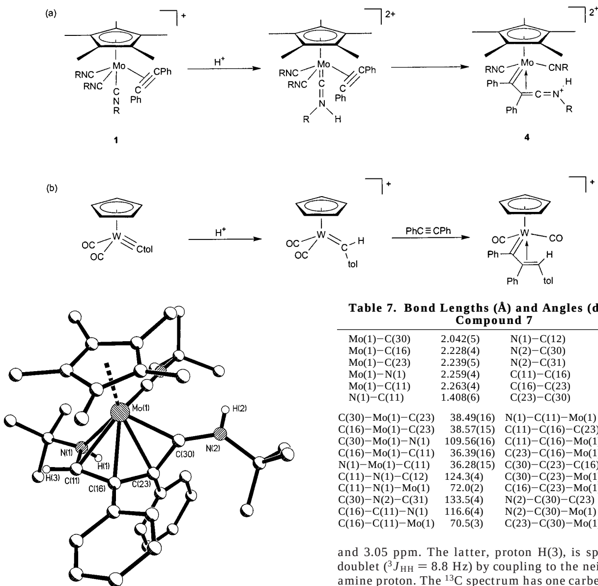
Figure 5. Structure of the cation of 7. Most hydrogen atoms have been omitted for clarity.
