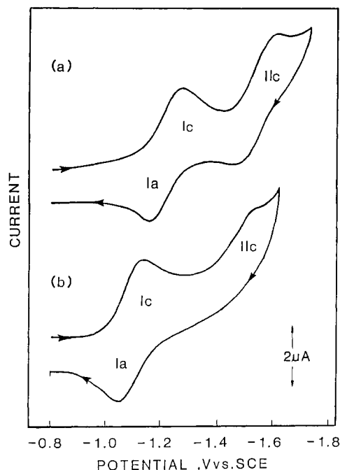
Figure 6. Cyclic voltammogram of PCPP: (a) in 1,2-dichloroethane containing 0.1 M TBAP and (b) in 1,2-dichloroethane containing 0.1 M TBAP and 1 \mu M of TEAH. Scan rate = 100 mV/s.
