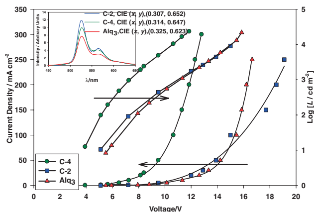
Figure 5. Current density–voltage–luminance characteristics of ITO/ZnTPP (50 nm)/ \alpha -NPB (50 nm)/Alq 3 :DPQA (50 nm:0.1 nm)/ETL (20 nm)/LiF (0.5 nm)/Al.
