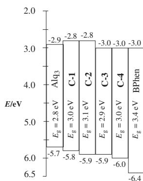
Figure 3. HOMO–LUMO energy levels of C-1–C-4 , Alq 3 , and BPhen.
