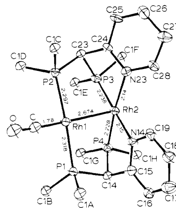
Figure 1. An ORTEP drawing of the dication of [\text{Rh}_2(\text{CO})(\mu\text{-PNP})_2](\text{BPh}_4)_2 \cdot 2\text{CH}_2\text{Cl}_2 . Phenyl carbon atoms have been omitted for clarity and are numbered C1A, C2A, ..., C6A for rings A-H. Some selected bond angles and distances are \text{Rh1-Rh2-P3} = 94.9 (1)^\circ , \text{Rh1-Rh2-P4} = 88.7 (1)^\circ , \text{Rh1-Rh2-N14} = 82.3 (3)^\circ , \text{Rh1-Rh2-N23} = 97.9 (3)^\circ , \text{Rh2-Rh1-P1} = 92.3 (1)^\circ , \text{Rh2-Rh1-P2} = 88.2 (1)^\circ , \text{Rh2-Rh1-C} = 166.5 (5)^\circ , \text{P1-Rh1-C} = 90.0 (5)^\circ , \text{P2-Rh1-C} = 91.2 (5)^\circ , \text{Rh1-C-O} = 176 (1)^\circ , and \text{C-O} = 1.18 (1) \text{ \AA} .
