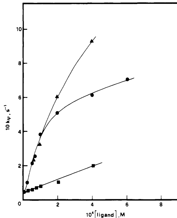
Figure 1. Rate vs concentration profiles for the cleavage of PNPP at different ligand concentrations in homoaggregates. Conditions: 0.05 M MES buffer (pH 6.3), 25 °C, [\text{Cu}^{2+}] = 1.8 \times 10^{-4} M. \Delta , ligand 1 ; \blacksquare , ligand 2 ; \bullet , ligand 3 .
