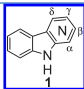
Figure 1. General structure of carbolines.
