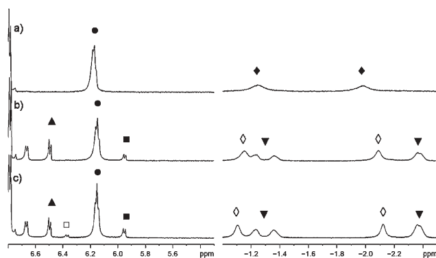
Fig. 3 Progress of S_NAr reaction between 4 and 6 in the presence of 1 as followed by ^1H NMR (600 MHz, d_{10} - p -xylene, 300 K). a) t = 0 , before addition of 6 ; b) t = 17 min; c) t = 98 min (●: methine protons of 1 vase; ◆: encapsulated 4 ; ▲: starting material 6 ; ■: aromatic proton of bound S_NAr product; □: aromatic proton of free product; ◇: bound 4 in fast exchange with protonated bound 4 ; ▼: encapsulated product).
