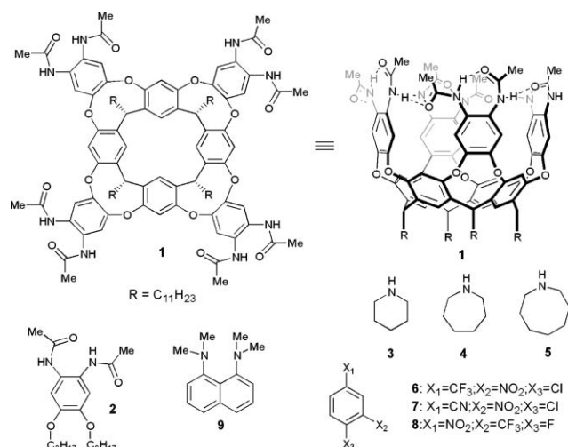
Fig. 1 Cavitand host, wall mimic, amine guests, and aromatic substrates.
