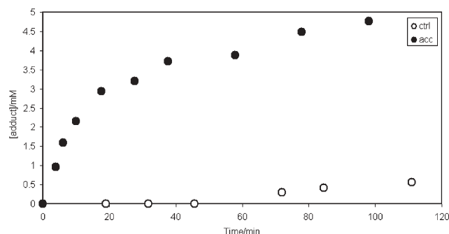
Fig. 4 Acceleration of S_NAr reaction between 4 and 6 with 1 . Conditions: [ 1 ] = 10 mM; [ 4 ] = 21 mM; [ 6 ] = 10 mM; [ 9 ] = 21 mM (○: background reaction (ctrl) in the absence of 1 ; ●: accelerated reaction (acc)).
