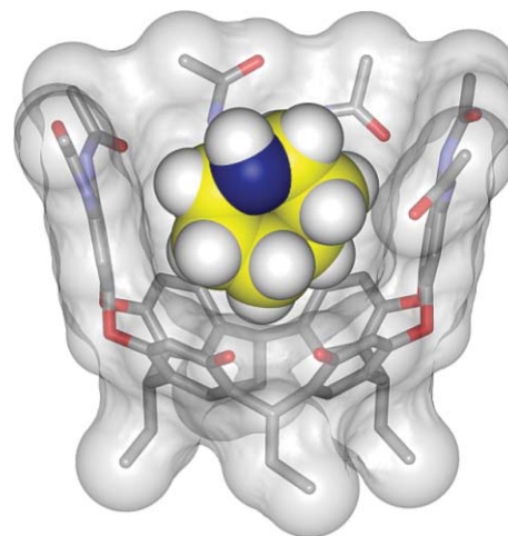
Fig. 2 Molecular model of encapsulated 4 with front cavitand wall removed for viewing ease (Spartan, molecular mechanics force field).
