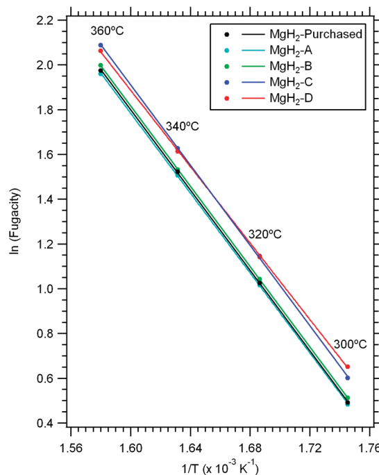
Figure 4. van't Hoff plot for the decomposition of MgH 2 in the four mechanochemically synthesized samples as well as the bulk reference (MgH 2 -Purchased).
