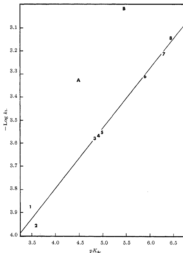
Figure 1.—Free energy plots of -\log k_1 vs. pK_a for the reaction of Cr(CO) 4 (X-o-phen) with P(OCH 2 ) 3 CCH 3 in 1,2-dichloroethane at 47.9°. The numbers represent the X-o-phen as listed in Table I. A and B represent the reactions of Cr(CO) 4 (dipy) and Cr(CO) 4 -(4,4'-dimethyldipy) with P(OCH 2 ) 3 CCH 3 .
