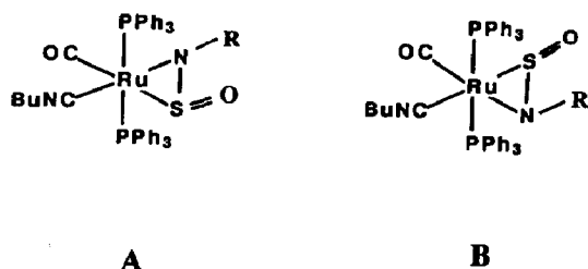
Scheme 3. R = C 6 H 4 Me- p .
