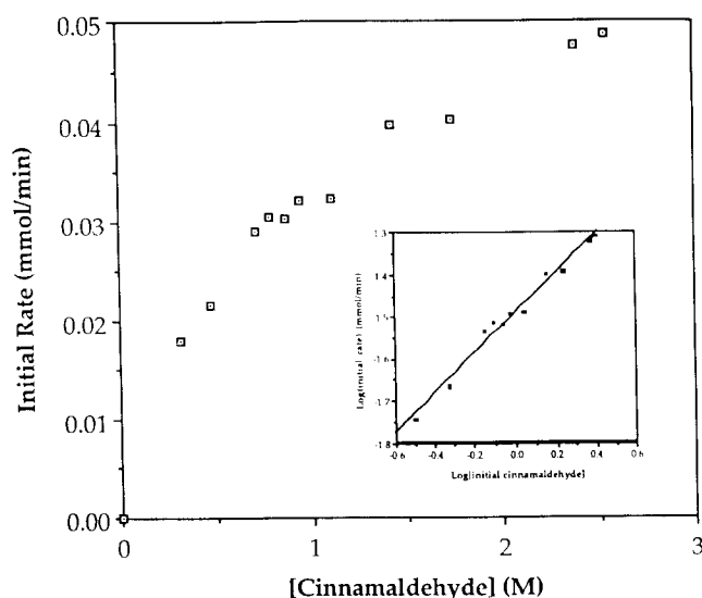
Fig. 4. Dependence of the rate on initial substrate concentration for the reduction of trans -cinnamaldehyde in the presence of complex 1 ( 9 \times 10^{-5} M) with aqueous \text{NaOOCH} (5 M) at 75°C. The insert shows the corresponding log-log plot, which provides a reaction order of 0.47.
