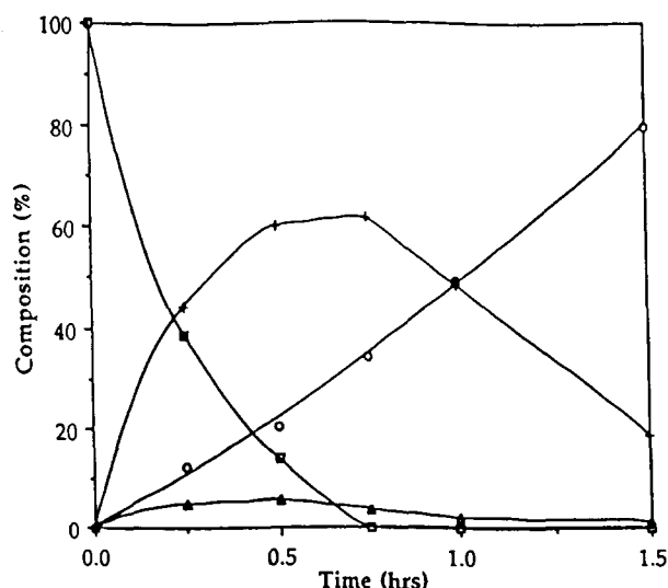
Fig. 5. Reaction profile for the reduction of allyl benzene (0.66 ml) in the presence of complex 1 (0.08 mmol) in 5 ml of 5 M formate buffer with H_2 at 50°C; \square allyl benzene, \circ propyl benzene, + trans -propenyl benzene, \Delta cis -propenyl benzene.
