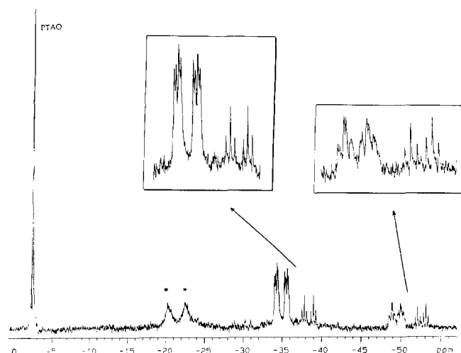
Fig. 6. ^{31}P NMR spectrum of the mixture formed in the reversible reaction of [Rh(PTAH)(PTA)_2Cl]Cl with H_2 . Peaks indicated by asterisks are caused by [Rh(PTAH)(PTA)_2Cl]Cl .
