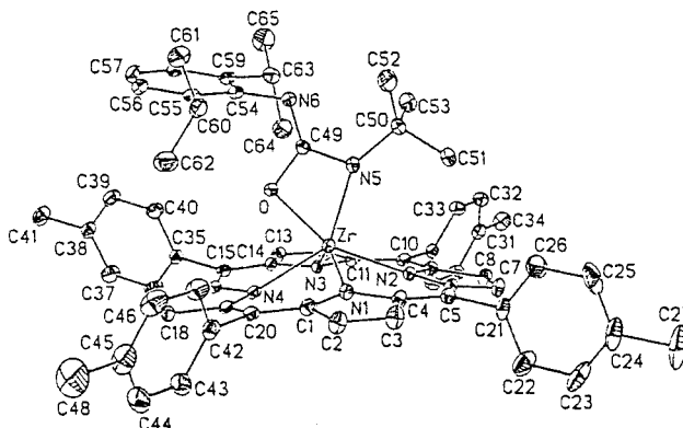
Figure 4. ORTEP representation of (\text{TTP})\text{Zr}(\eta^2\text{-N}^t\text{BuC}(=\text{NAr}^{\text{iPr}})\text{O}) . Thermal ellipsoids are drawn at the 30% probability level.
