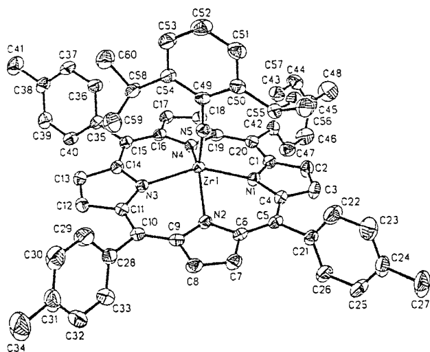
Figure 1. ORTEP representation of (TTP)Zr=NAr iPr . Thermal ellipsoids are drawn at the 50% probability level.
