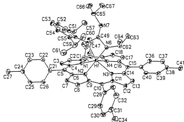
Figure 5. ORTEP representation of (\text{TTP})\text{Hf}(\eta^2\text{-NAr}^{\text{iPr}}\text{C}(=\text{N}^{\text{iPr}})\text{N}^{\text{iPr}}) . Thermal ellipsoids are drawn at the 30% probability level.
