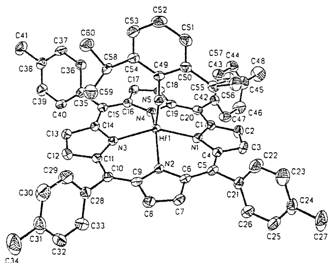
Figure 2. ORTEP representation of (TTP)Hf=NAr iPr . Thermal ellipsoids are drawn at the 50% probability level.
