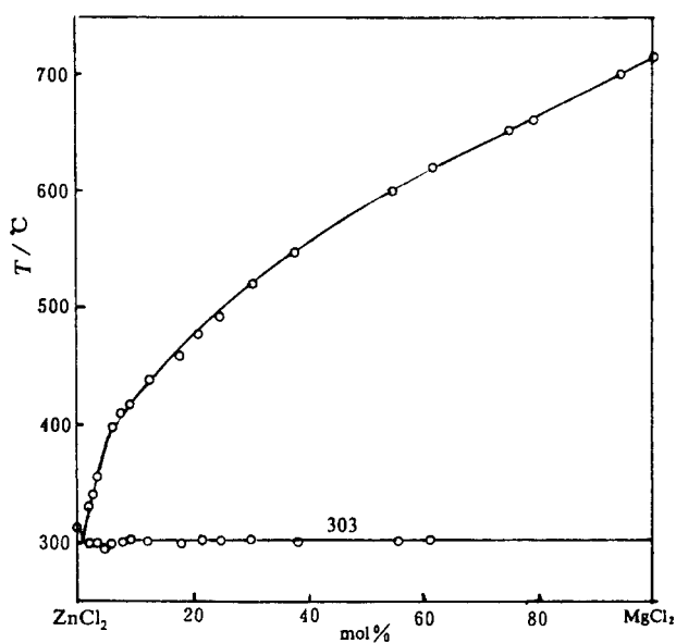
Fig. 2. Phase diagram of the \text{ZnCl}_2 - \text{MgCl}_2 system.
