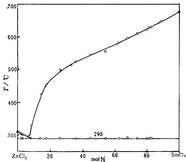
Fig. 1. Phase diagram of the \text{SmCl}_3 - \text{ZnCl}_2 system.
