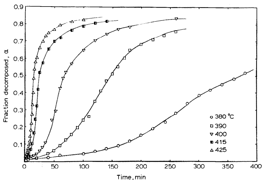
Fig. 2. Thermal decomposition of 100 Mrad \gamma -irradiated lead nitrate at different temperatures.
