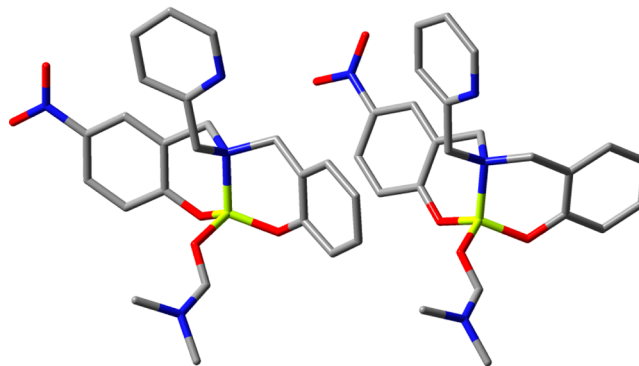
Figure 5. Optimized models of the syn (left) and anti (right) [\text{Be}(\mathbf{2a})(\text{DMF})] complexes. \text{Be}^{\text{II}} is yellow, O is red, N is blue, and C is gray. Hydrogen atoms have been removed for clarity.
