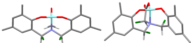
Figure 2. Geometry-optimized syn conformer (left) and anti conformer (right) of 3g . \text{Be}^{\text{II}} is light blue, O is red, N is blue, and C is gray. Equatorial protons are shown in green for clarity.
