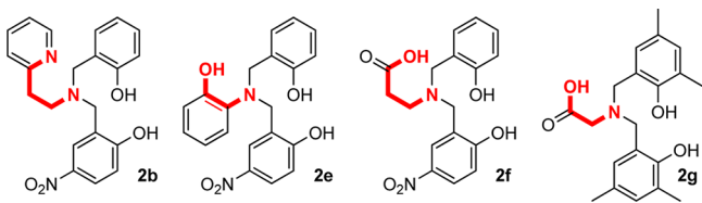
Figure 3. Tetracoordinate ligands with well-correlated ^9\text{Be} NMR shifts upon \text{Be}^{\text{II}} coordination.
