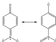
Figure 6. Resonance structures of 4-nitrophenolate.
