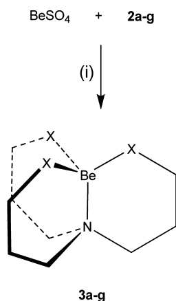
Scheme 2. Generalized Structure for the Be II Tetracoordinate Complexes 3a–g a
