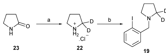
Scheme 13 Reagents and conditions: (a) \text{LiAlD}_4 (2.5 equiv.), THF, 0^\circ\text{C} then 67^\circ\text{C} , 14 h, then \text{HCl} , \text{H}_2\text{O} (62%); (b) 2-iodobenzyl bromide (1.1 equiv.), \text{PrNEt}_2 (4.0 equiv.), \text{CH}_3\text{CN} , rt, 14 h (53%).
