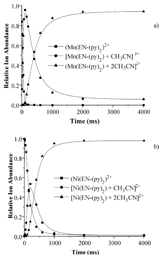
Figure 4. Kinetic plots for the reactions of (a) \text{Mn}(\text{EN}(\text{py})_2)^{2+} and (b) \text{Ni}(\text{EN}(\text{py})_2)^{2+} with \text{CH}_3\text{CN} .
