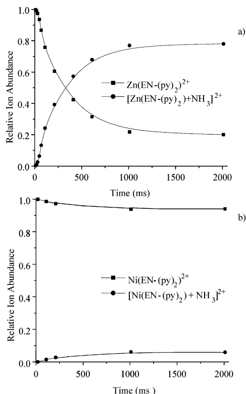
Figure 2. Typical kinetic plots obtained from the reactions of \text{NH}_3 with (a) \text{Zn}(\text{EN}(\text{py})_2)^{2+} and (b) \text{Ni}(\text{EN}(\text{py})_2)^{2+} .
