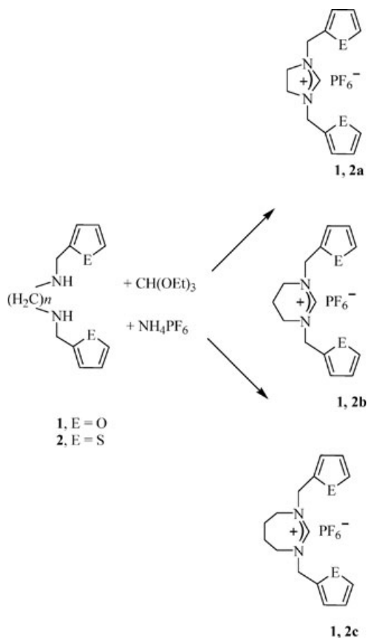
SCHEME 1 Synthesis of 1,3-dialkylazolinium salts (LHX).
