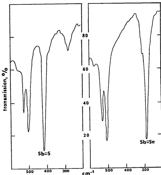
Fig. 1. (a) Infrared spectrum of triethylstibine sulfide (Nujol mull, polyethylene cells) and (b) of triethylstibine selenide (Nujol mull, polyethylene cells) in the region 200–700 \text{cm}^{-1} .
