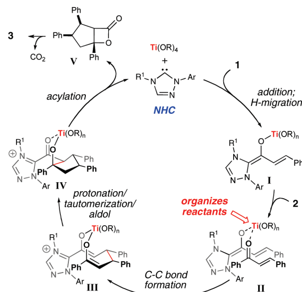
Scheme 1. Proposed Catalytic Pathway
