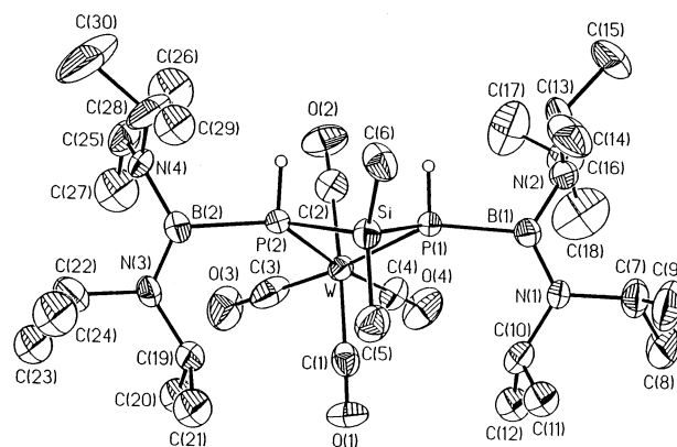
Fig. 2. Molecular structure and atom labeling scheme for [( i Pr 2 N) 2 BP(H)] 2 SiMe 2 ·W(CO) 4 5' (30% thermal ellipsoids).
