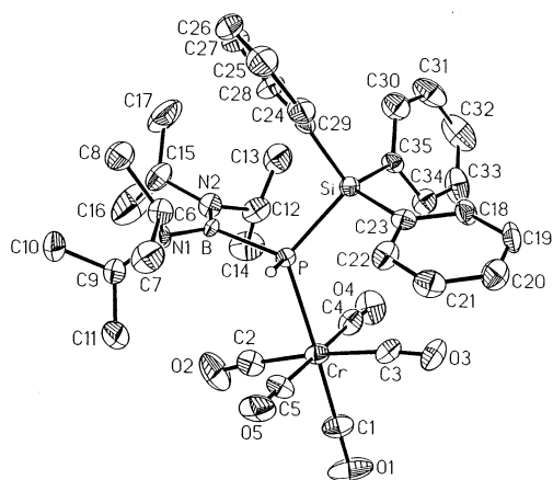
Fig. 1. Molecular structure and atom labeling scheme for ( i Pr 2 N) 2 BP(H)SiPh 3 ·Cr(CO) 5 , 4 (30% thermal ellipsoids).
