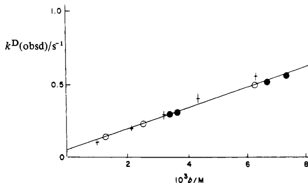
Figure 1. Plot of first-order rate constant k^{\text{D}}(\text{obsd}) against concentration b of TMG. Comparison of deuterated base (BD) with undeuterated (BH). The values reported for BD in ref 3 lie considerably higher. ●, BH (Mateo 1 ); ○, BH (this work); +, BD (this work). Horizontal axis, 10^3 b / \text{M} ; vertical axis: k^{\text{D}}(\text{obsd}) / \text{s}^{-1} .
