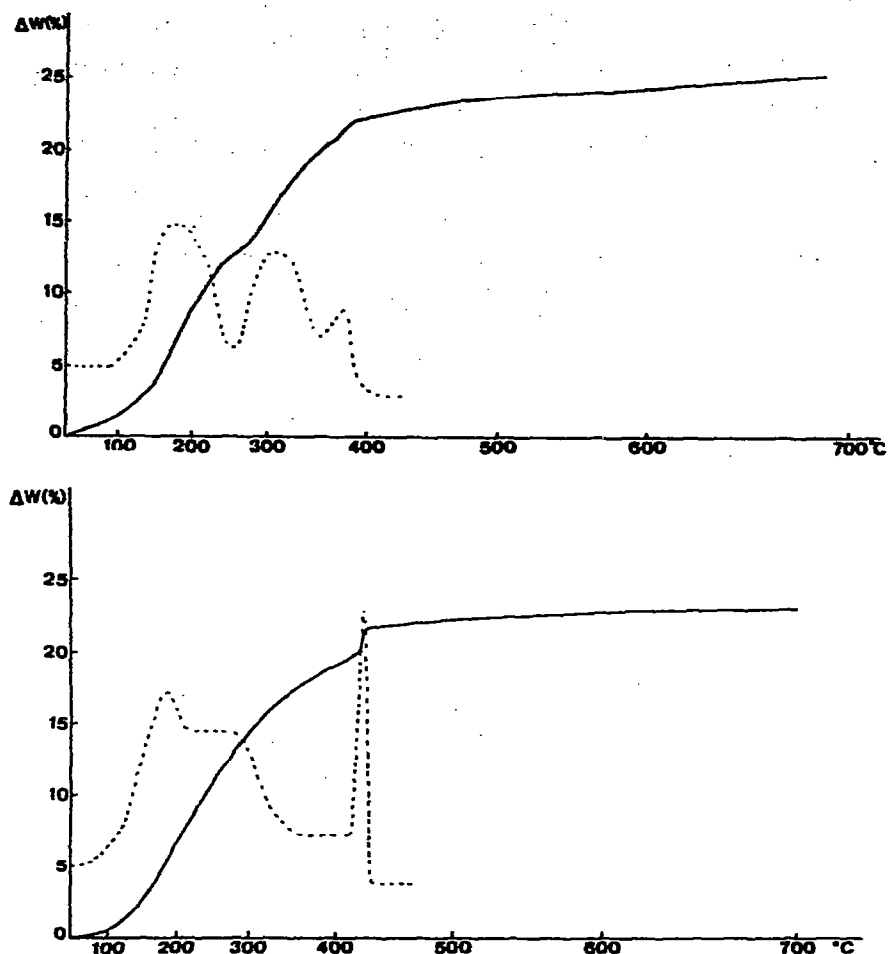
Fig. 4. (a) ———, TG curve of Ru(III) hydrate; ·····, differential curve. In air. (b) ———, TG curve of Ru(III) hydrate; ·····, differential curve. In nitrogen.
