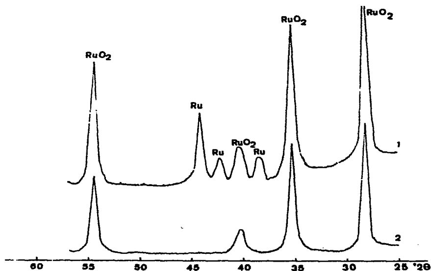
Fig. 3. X-Ray diffraction of Ru(III) hydrate heated at 500^\circ\text{C} in 1, nitrogen; and 2, air.
