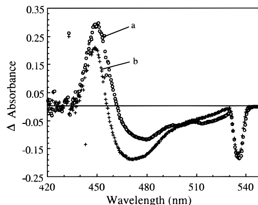
Figure 2. Transient absorption difference spectra of TPPFe II NO taken at (a) 10 and (b) 40 ps. The negative-going signals centered at 532 nm were due to scattered excitation light (532 nm).
