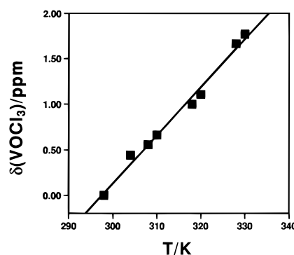
Figure 4. The chemical shift for the reference compound \text{VOCl}_3 (0.00 ppm, 298 K) is shown at variable temperatures.
