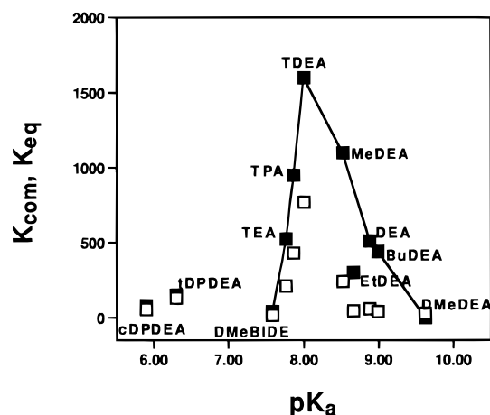
Figure 3. The composite pH-dependent and -independent formation constants K_{\text{com}} ( \square ) and K_{\text{eq}} ( \blacksquare ) plotted as a function of the \text{pK}_a of the protonated amine.
