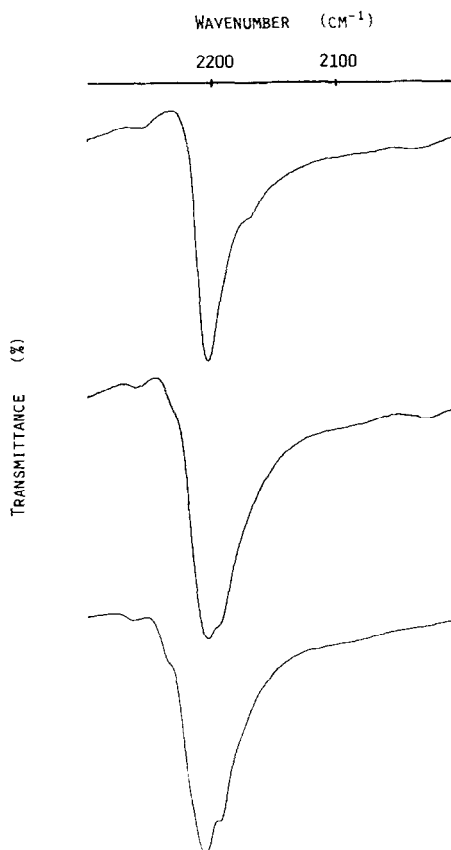
Fig. 1. The \nu(-N\equiv C) pattern (nujol/NaCl, 2300 – 2000\text{ cm}^{-1} ) for [\text{Co}(\text{CNR})_4](\text{ClO}_4)_2 , [\text{Co}(\text{CNR})_5](\text{ClO}_4)_2 \cdot 0.5\text{H}_2\text{O} , and [\text{Co}(\text{CNR})_5](\text{BF}_4)_2 \cdot 0.5\text{H}_2\text{O} (top to bottom, respectively), where R = 2,6\text{-Me}_2\text{C}_6\text{H}_3 .
