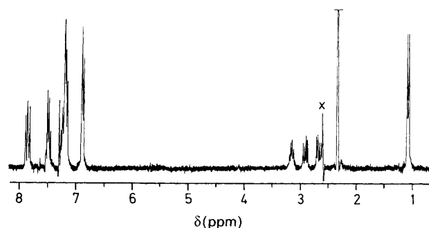
Figure 3. 270 MHz ^1\text{H} NMR difference spectrum obtained in deuteriochloroform at -50^\circ\text{C} , showing the spectrum of atropisomer (1b); peak labelled 'X' is a subtraction spike.
