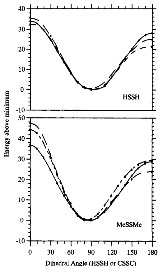
Figure 2. Relative energy (kJ/mol) of HSSH and MeSSMe as a function of the dihedral angle (HSSH or CSSC): (—) MM2(85) (this work); (---) 6-31G* (Aida); (-.-) SCF and MP2 (Marsden); (---) OPLS (Jorgensen).
