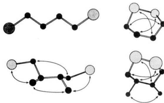
Figure 7. Gauche interactions in 27^{\text{red}} (BDT), 25^{\text{red}} , 27 (BDT ox ), and 25 .
