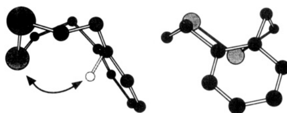
Figure 9. The most stable conformation of 52 . In 53 , hydrogen atoms of methylene units project into the crease of the molecule (relative position in light gray) and experience van der Waals repulsion. These hydrogen atoms and unfavorable interactions have been eliminated in 51 and 52 .
