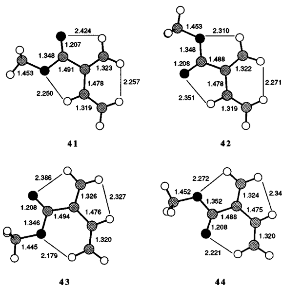
Fig. 1 RHF/3-21G optimised conformations of 2-methoxycarbonylbuta-1,3-diene
