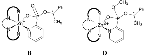
Figure 15. Tetradentate zinc complexes with TSA 13 ( B ) and a phosphodiester ( D ).
