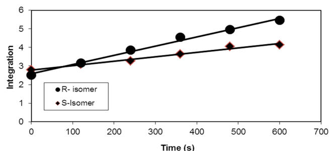
Figure 14. Time-dependent \text{PhCH}(\text{OD})\text{Me} formation in reaction of R - and S -1 in \text{CD}_3\text{OD}/\text{CD}_2\text{Cl}_2 (1:1) with 1 mol % [2-6-6]\text{Zn}(\text{OTf})_2 .
