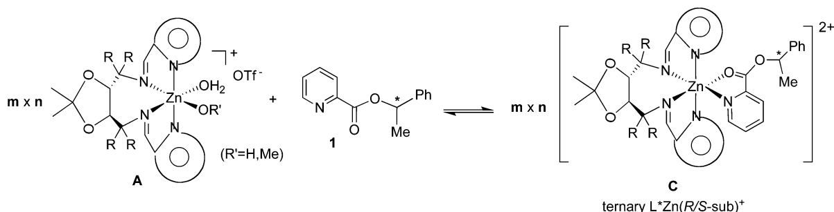
Figure 10. Formation of ternary \text{LZn}(\text{substrate})^+ complexes.
