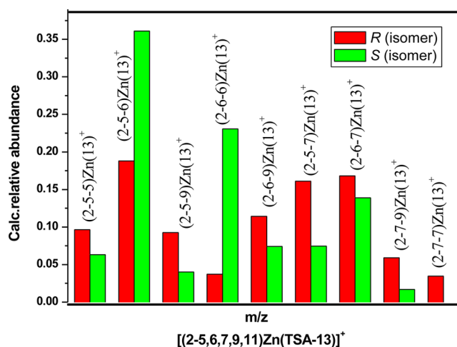
Figure 9. Amplification of \text{LZn}(13)^+ from (2-5, -6, -7, -9, -11) \text{Zn}(\text{OTf})_2 + R- or S-13 analyzed by ESI-MS at 24 h. The calculated relative abundance = (ion count of peak/ion count of internal standard)/sum over all ions of (ion count of peak/ion count of internal standard).
