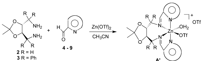
Figure 11. Preparation of isolable binary \text{LZn}(\text{OTf})^+ complexes.
