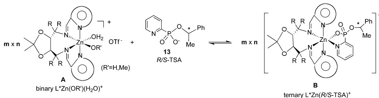
Figure 5. Formation of ternary LZn(TSA)^+ complexes.
