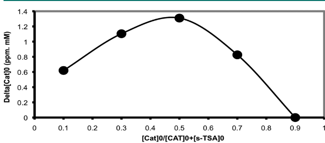
Figure 6. Job plot for the complexation (2-6-6)Zn(OTf)^+ with S -TSA ( 13 ) at a total concentration of 10 mM in CD_3OD ; weighted value of imine proton NMR chemical shift \delta \times complex concentration [mM] (x-axis) as a function of [cat]^0/[cat]^0+[S-TSA]^0 (y-axis).
