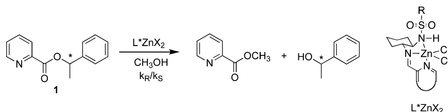
Figure 2. LZnX 2 -catalyzed methanolysis of chiral picolinate ester.
