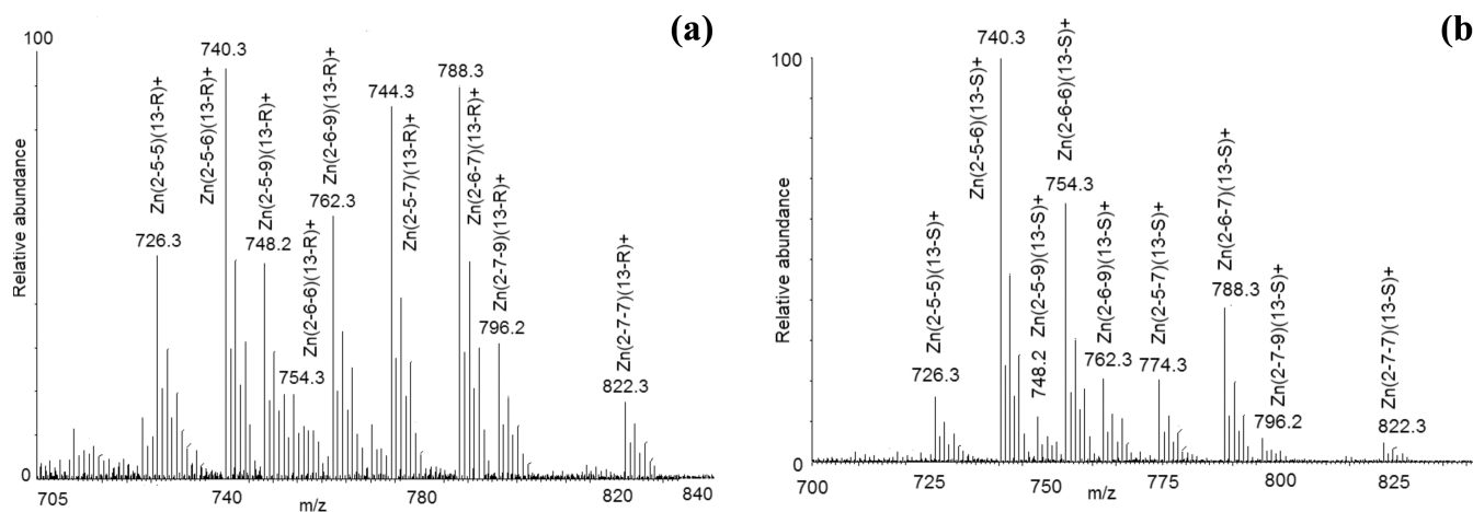
Figure 8. Portion of ESI-MS of (a) (2-5, -6, -7, -9, -11) \text{Zn}(\text{OTf})_2 + R-13; and (b) (2-5, -6, -7, -9, -11) \text{Zn}(\text{OTf})_2 + S-13; at 24 h in MeOH.
