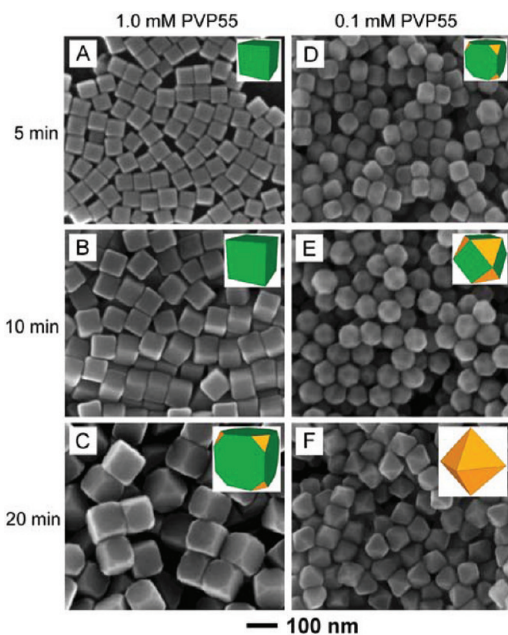
Figure 2. SEM images of Ag polyhedrons grown from 40 nm cubic seeds in the presence of (A–C) 1.0 mM and (D–F) 0.1 mM PVP55, respectively, as the capping agent. The samples were collected from the reaction solutions at different time points: (A, D) 5 min, (B, E) 10 min, and (C, F) 20 min. The inset shows the corresponding 3D model for each type of polyhedron.
