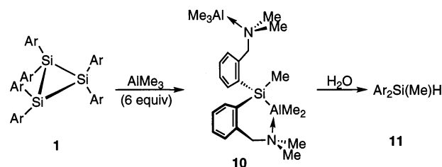
Scheme 3. Synthesis and hydrolysis of 10 ; Ar = 2-(Me 2 NCH 2 )C 6 H 4 .
