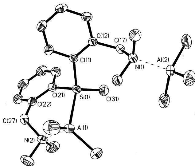
Fig. 2. Crystal structure of 10 . Hydrogen atoms are omitted for clarity, displacement ellipsoids are at the 50% probability level. Selected bond lengths (pm) and bond angles (°): Si(1)–Al(1) 247.5(1), Si(1)–C(11) 191.5(2), Si(1)–C(21) 191.1(2), Si(1)–C(31) 189.8(3), Al(1)–N(2) 205.5(2), Al(2)–N(1) 205.7(2); Al(1)–Si(1)–C(11) 118.23(7), Al(1)–Si(1)–C(21) 106.99(7), Al(1)–Si(1)–C(31) 113.13(8), C(11)–Si(1)–C(21) 102.42(9), C(11)–Si(1)–C(31) 112.2(1), C(21)–Si(1)–C(31) 101.6(1).
