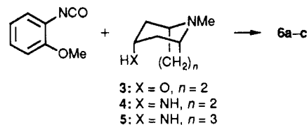
Scheme I. Synthesis of Ureas 6a–c
