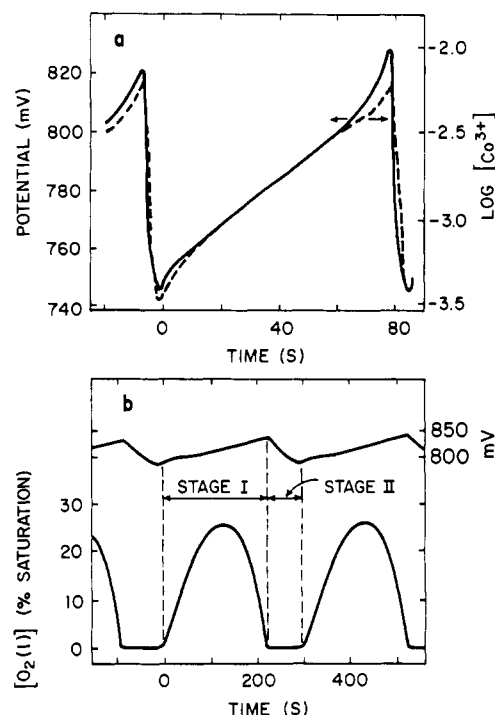
Figure 1. (a) Oscillations of the platinum electrode potential vs. Ag/AgCl reference electrode (—) and \log [Co^{3+}] determined by optical absorption at 620 nm (---). A 150-mL solution contained initially 500 nM PhCHO, 10 mM Co(AcO)_2 , 5 mM NaBr, and 90/10 w/w AcOH/ H_2O as solvent. The temperature was 70 °C, an O_2 pressure of 580 torr was maintained above the solution, and the magnetic stirring speed was 400 rpm. (b) A comparison of the Pt electrode response (top trace) with the dissolved oxygen concentration (bottom trace) expressed in terms of the percentage of saturation with O_2 at a partial pressure of 580 torr. We estimate that 100% on this scale corresponds to [O_2(l)] = 5 \pm 2 mM. Conditions are as in (a), but the solution contained initially 750 mM PhCHO, 20 mM Co(AcO)_2 , and 2 mM NaBr; O_2 was introduced at a flow rate of 20 mL/min through a frit immersed in the liquid.
