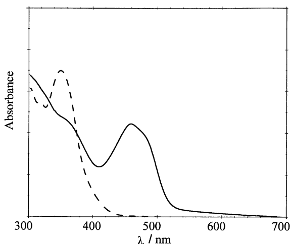
Figure 3. Electronic spectra of 2 . Solid line: in a thin KBr disk, \lambda_{\max} = 460 nm. Broken line: in 3-methylpentane, \lambda_{\max} = 350 nm, \epsilon = 9.94 \times 10^3 ( c = 7.05 \times 10^{-5} mol L ^{-1} ).
