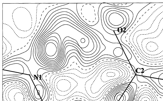
Figure 2. A difference electron density map in the plane of N(1)-C(2)-O(2) at 90 K. Contour interval 0.05 eÅ -3 , negative contours dotted, zero contour dashed, positive contours solid.
