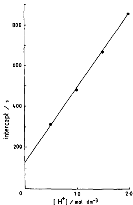
Fig. 5. Plot of the intercept (s) of k_0^{-1} vs. [\text{Br}^-]^{-1} against [\text{H}^+] ( \text{mol dm}^{-3} ) at an ionic strength of 2.00 \text{ mol dm}^{-3} at 21.8^\circ\text{C} .
