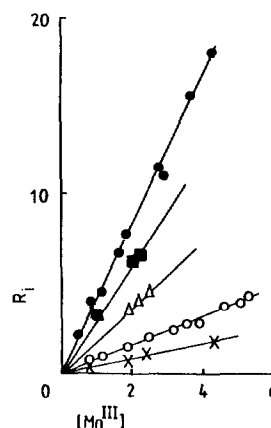
Fig. 1. Plots of R_i ( 10^{-5} \text{ mol dm}^{-3} \text{ s}^{-1} ) against initial [\text{Mn}(\text{bipy})_2^{3+}] ( 10^{-4} \text{ mol dm}^{-3} ) for the oxidation of bromide ions at [\text{H}^+] = 0.20 \text{ mol dm}^{-3} and at an ionic strength = 1.00 \text{ mol dm}^{-3} and at 21.8 °C with [\text{Br}^-] ( 10^{-3} \text{ mol dm}^{-3} ) as follows: x, 4.00; o, 8.00; Δ, 16.0; ■, 30.0; ●, 40.0.
