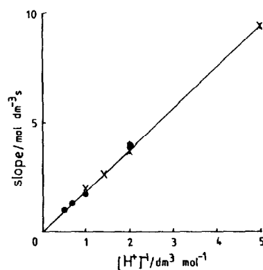
Fig. 4. Plot of the slope (mol dm -3 s) against [\text{H}^+]^{-1} (dm 3 mol -1 ) for k_0^{-1} vs. [\text{Br}^-]^{-1} at ionic strengths of 1.00 (X) and 2.00 (●) (mol dm -3 ) at 21.8 °C.
