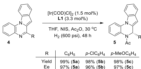
Scheme 3. Substrate scope: indolo[1,2- a ]quinoxalines.
