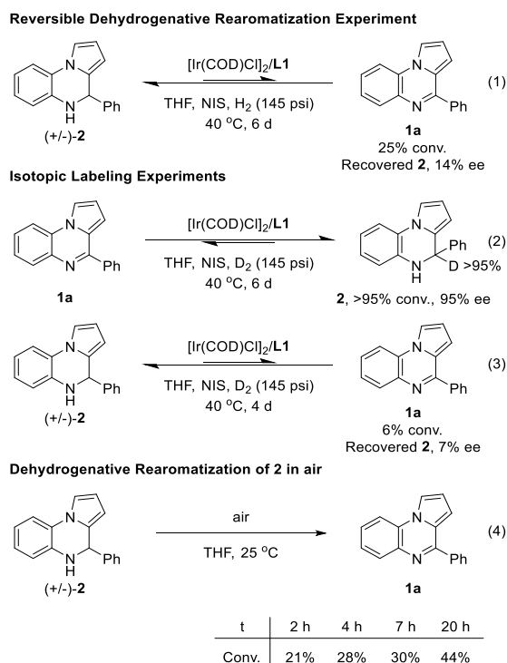
Scheme 2. Rearomatization experiments of 2 .
