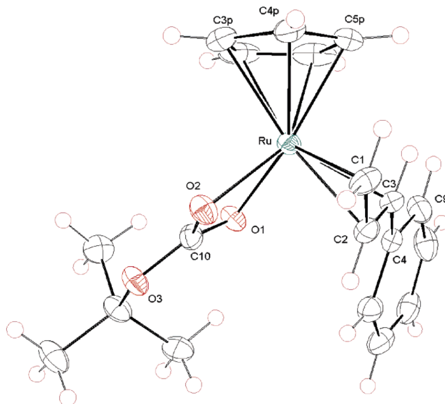
Figure 3. ORTEP view of the Ru(II) cationic complex 7b . The PF 6 anion is omitted for clarity.
