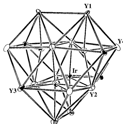
Figure 13. The \text{Y}_{16}\text{Ir}_4 cluster ( \bar{4} symmetry) in \text{Y}_{20}\text{Br}_{36}\text{Ir}_4 with four crystallographically distinct Y atoms indicated. \bar{a} is horizontal; \bar{c} is vertical.
