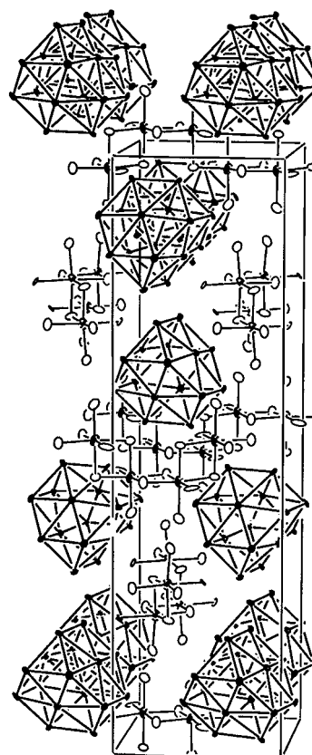
Figure 12. [\bar{1}00] view of the tetragonal unit cell in \text{Y}_{20}\text{Br}_{36}\text{Ir}_4 , illustrating the body-centered nature of the cluster packing. The structure is built of \text{Y}_{16}\text{Ir}_4 clusters and \text{YBr}_{4/2}^{\text{ch}}\text{Br}_{2/2}^{\text{cl}} chains. For clarity, only Br atoms (open ellipsoids) in the latter chains are pictured. \bar{b} is horizontal; \bar{c} is vertical.
