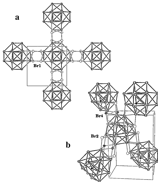
Figure 5. Intercluster bonding in \text{Y}_{16}\text{Br}_{20}\text{Ru}_4 (a) via Br1 atoms to form a square network within the a - b plane and (b) via \text{Br}^{2i-a} and \text{Br}^{4i-i} (dotted) atoms in a pseudotetrahedral arrangement of clusters along \bar{c} . \bar{b} is horizontal in both views.
