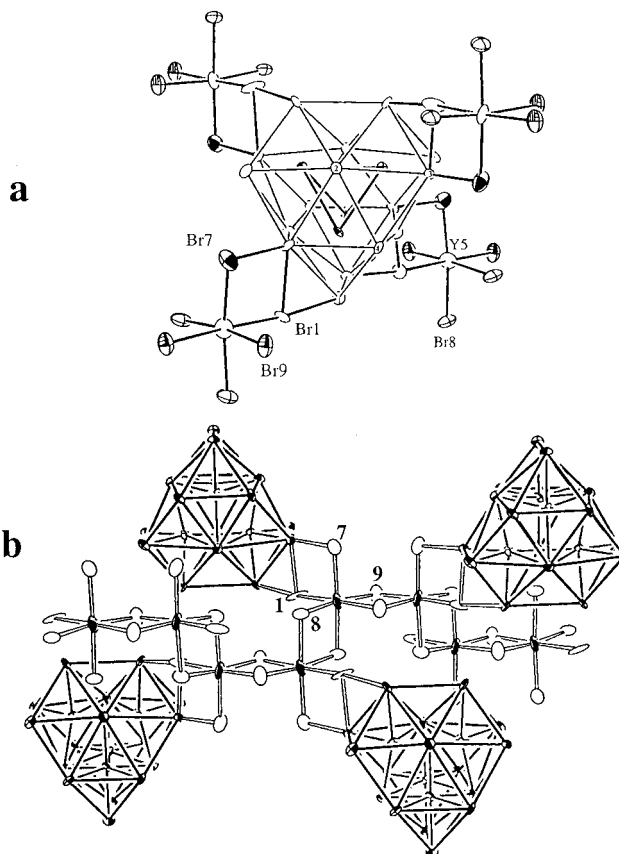
Figure 16. (a) 0\bar{1}0 view of the bonding between the clusters and the \text{YBr}_{4/2}\text{BrCl}_{2/2} chains in \text{Y}_{20}\text{Br}_{36}\text{Ir}_4 . Br1 bridges the Y1—Y3 cluster edges while bonding to the isolated Y5, and Br7 is exo to both a Y3 vertex and the Y5 atom. Pairs of Br8 and Br9 bond exclusively within the chain, bridging cis edges of the Y5-centered octahedron ( \bar{a} is horizontal). (b) The cluster-chain interconnectivity along the zigzag \text{YBr}_{4/2}\text{BrCl}_{2/2} chains. Clusters are alternately connected on both sides of and above and below the chain.
