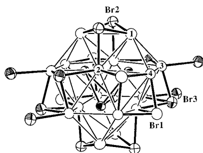
Figure 8. [110] view of three bonding modes of bromine in Y_{16}Br_{24}Ir_4 . Br1 and Br2 cap triangular faces ( Y2-Y4-Y4 and Y2-Y1-Y1 , respectively) on only one cluster, while Br3 caps Y2-Y3-Y3 faces and bonds exo to Y3 in another.
