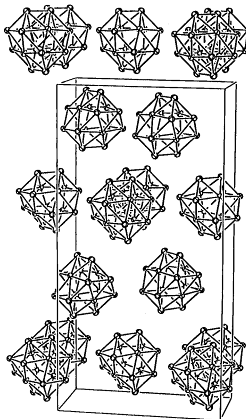
Figure 6. \sim[100] view of the unit cell of orthorhombic \text{Y}_{16}\text{Br}_{24}\text{Ir}_4 illustrating the face-centered nature of the cluster packing. \bar{b} is horizontal; \bar{c} is vertical. All Br and Ir atoms are omitted for clarity.
