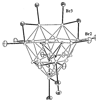
Figure 15. Bonding of Br2 and Br3 atoms in \text{Y}_{20}\text{Br}_{36}\text{Ir}_4 which bridge the Y3—Y4 and Y1—Y4 edges, respectively, while bonding exo to Y4 vertices in adjacent clusters (Y labels as in Figure 13).
