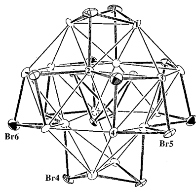
Figure 14. Bonding modes of Br4, Br5, and Br6 in \text{Y}_{20}\text{Br}_{36}\text{Ir}_4 which cap triangular faces (Y1—Y2—Y1, Y2—Y3—Y4, and Y2'—Y3—Y4, respectively) within the hexagon about Y2 on only one cluster. \bar{a} is horizontal; \bar{c} is vertical.
