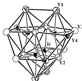
Figure 7. [110] view of a \text{Y}_{16}\text{Ir}_4 cluster unit in \text{Y}_{16}\text{Br}_{24}\text{Ir}_4 with the four types of Y atoms indicated ( \bar{c} vertical; 222 ( D_2 ) symmetry). Compare Figure 1a.
