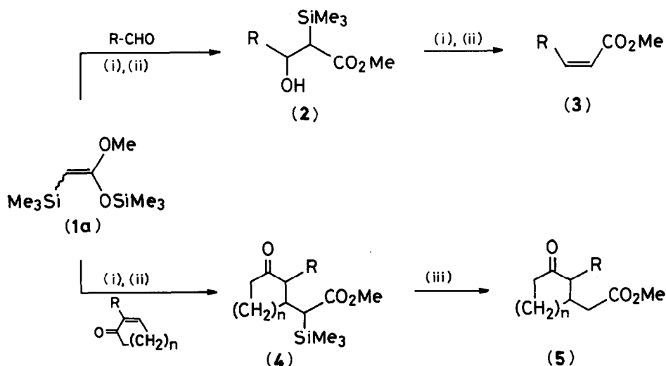
SCHEME 1. (i) TiCl 4 /CH 2 Cl 2 , -78°C. (ii) aq. K 2 CO 3 . (iii) KF/aq. MeOH, room temperature.
